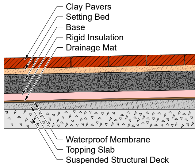
Figure 5 Typical Suspended Deck Paving Section
