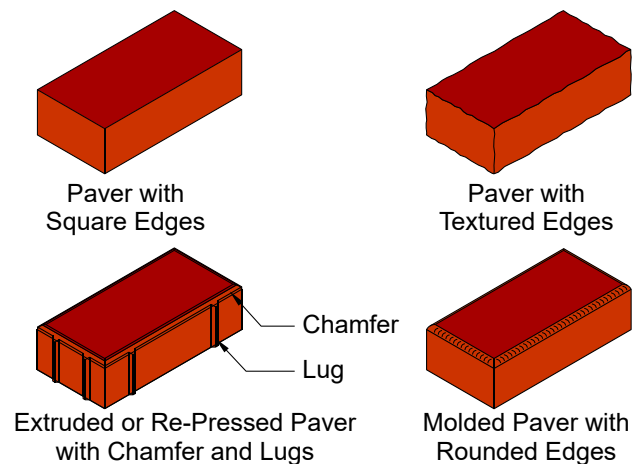
Figure 4 Clay Pavers
