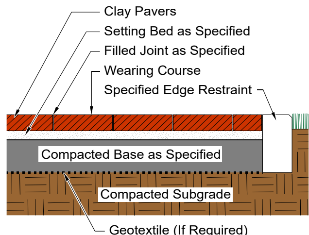
Figure 1 Typical Pavement Section
